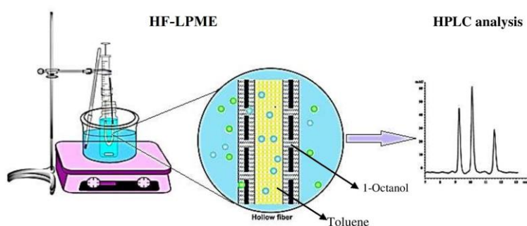
Fig. 1. Schematic diagram of the HF-LPME system
